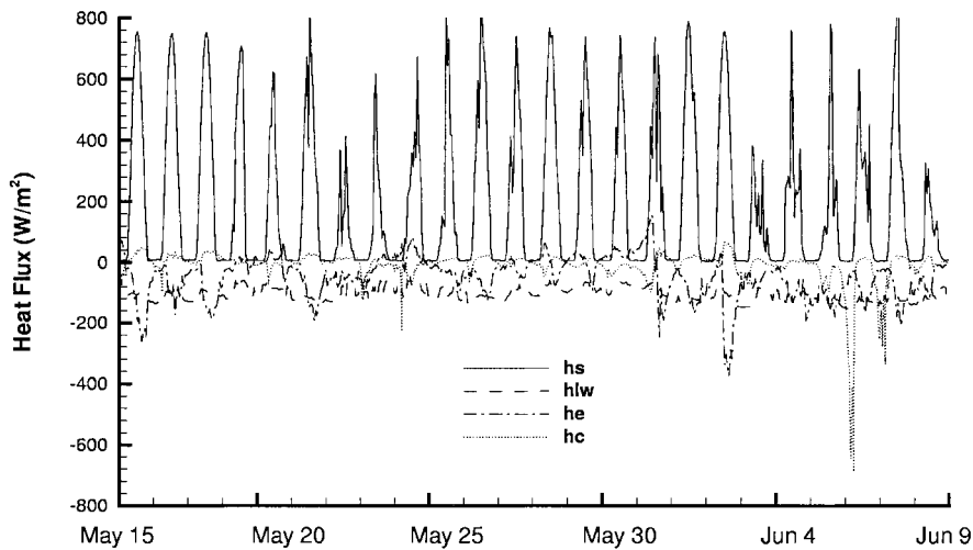
FIG. 11. Comparison among Computed Heat Flux Components ( \text{W}/\text{m}^2 ) of Solar (Shortwave) Radiation ( h_s ), Longwave Radiation ( h_{lw} ), Evaporation ( h_e ), and Convection ( h_c ) from May 15 to June 9, 1998, at Downstream Gauging Station on Little Pine Creek
