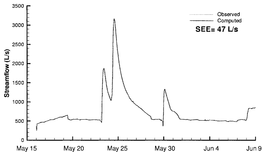
FIG. 5. Comparison of Measured Streamflow (L/s) with Simulated Streamflow (L/s) from May 15 to June 9, 1998, at Downstream Gauging Station on Little Pine Creek
