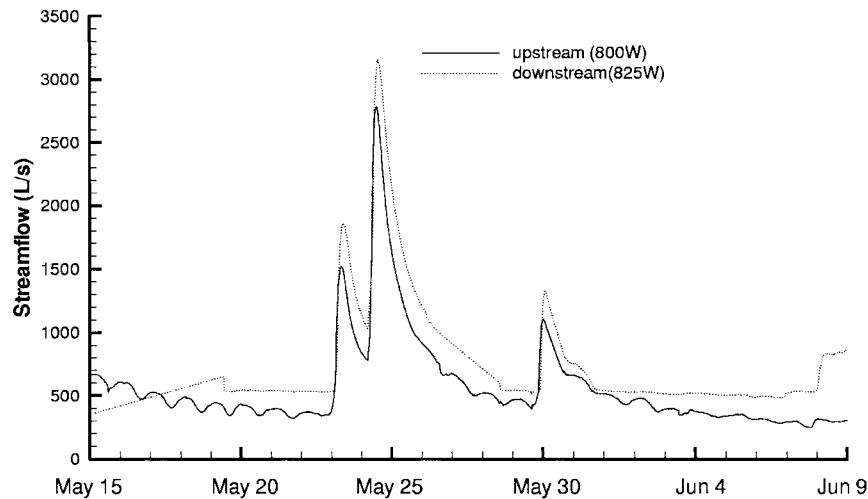
FIG. 4. Measured Short-Term Streamflow (L/s) from May 15 to June 9, 1998, at Stream Gauges on Little Pine Creek
